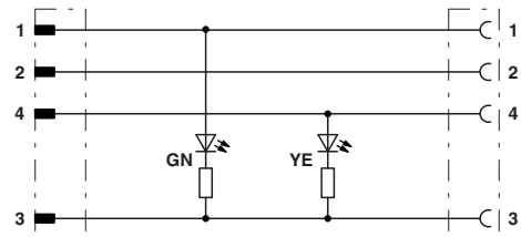
Contact assignment of M12 plugs / M8 sockets
